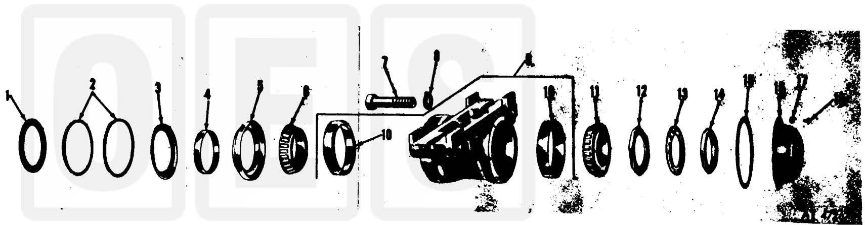
Figure 126. Rear spring seat and bearing.
